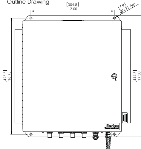
Outline Drawing
