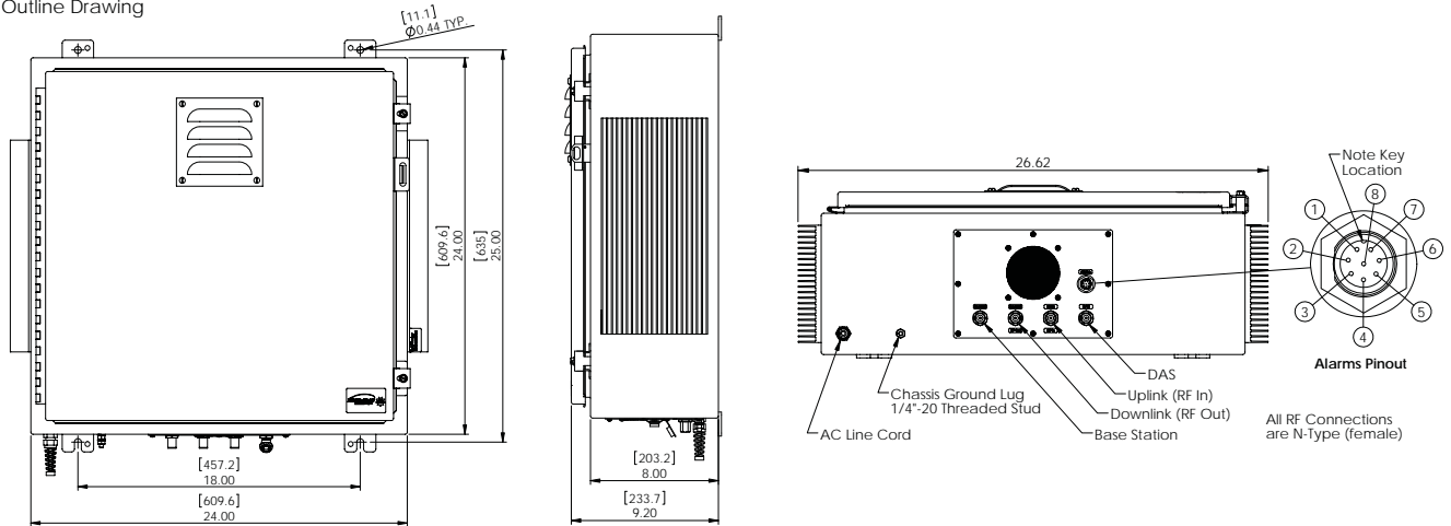
Outline Drawing
